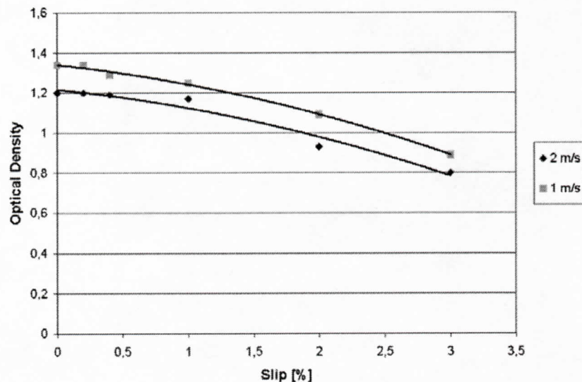
Figure 3: optical density vs. slip
