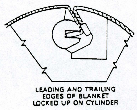
Figure 14. Single reel rod lockup system
