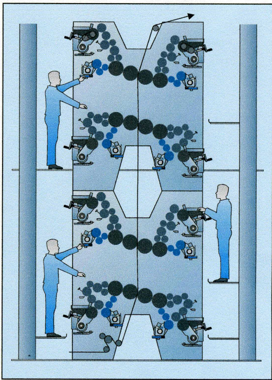
Figure 2-7. The vertically arranged printing unit of a CROMOMAN web press for four-page newspaper printing. (Courtesy MAN Roland Druckmaschinen AG)
