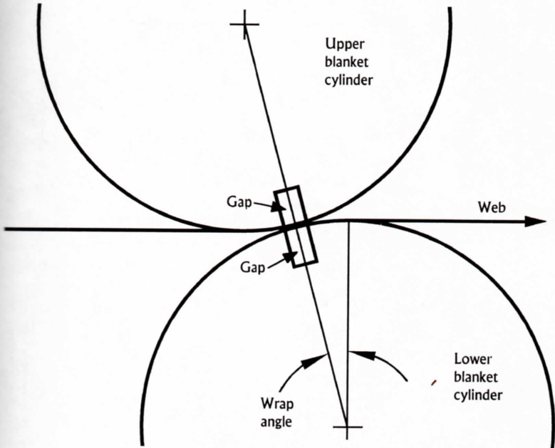
Figure 6.10 Web wrap achieved by canting the line connecting blanket cylinder centers.
