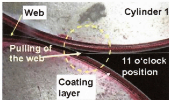
Fig. 3: The influence of cylinder orientation on web movement and cause of ghosting
